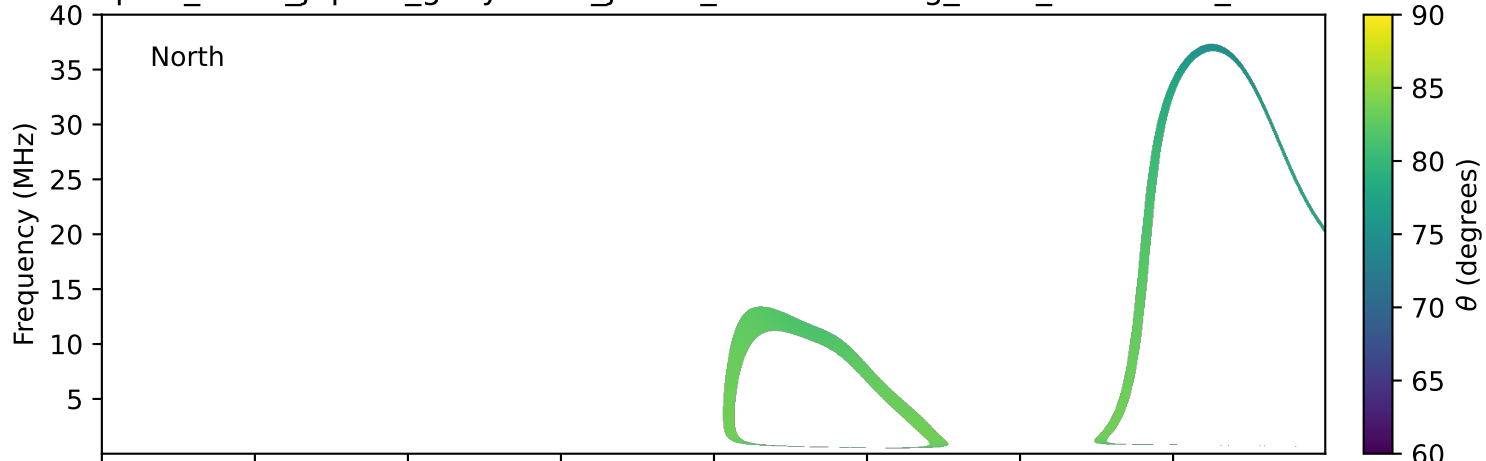
expres_earth_jupiter_ganymede_jrm33_lossc-wid1deg_3kev_20020617_v11.cdf
