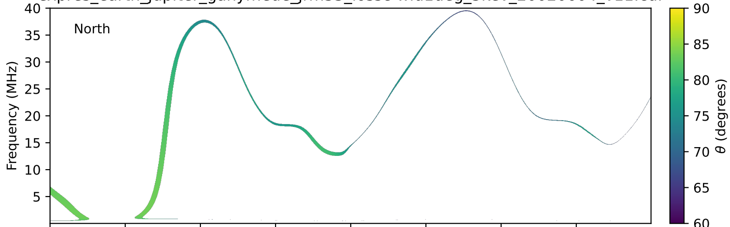
expres_earth_jupiter_ganymede_jrm33_lossc-wid1deg_3kev_20020604_v11.cdf
