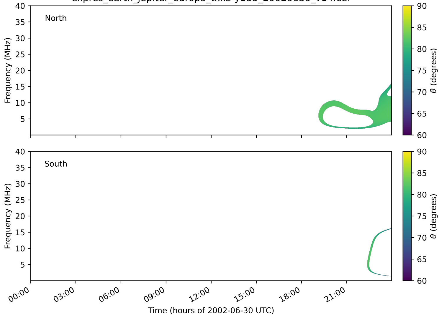
expres_earth_jupiter_europa_txka-y235_20020630_v14.cdf
