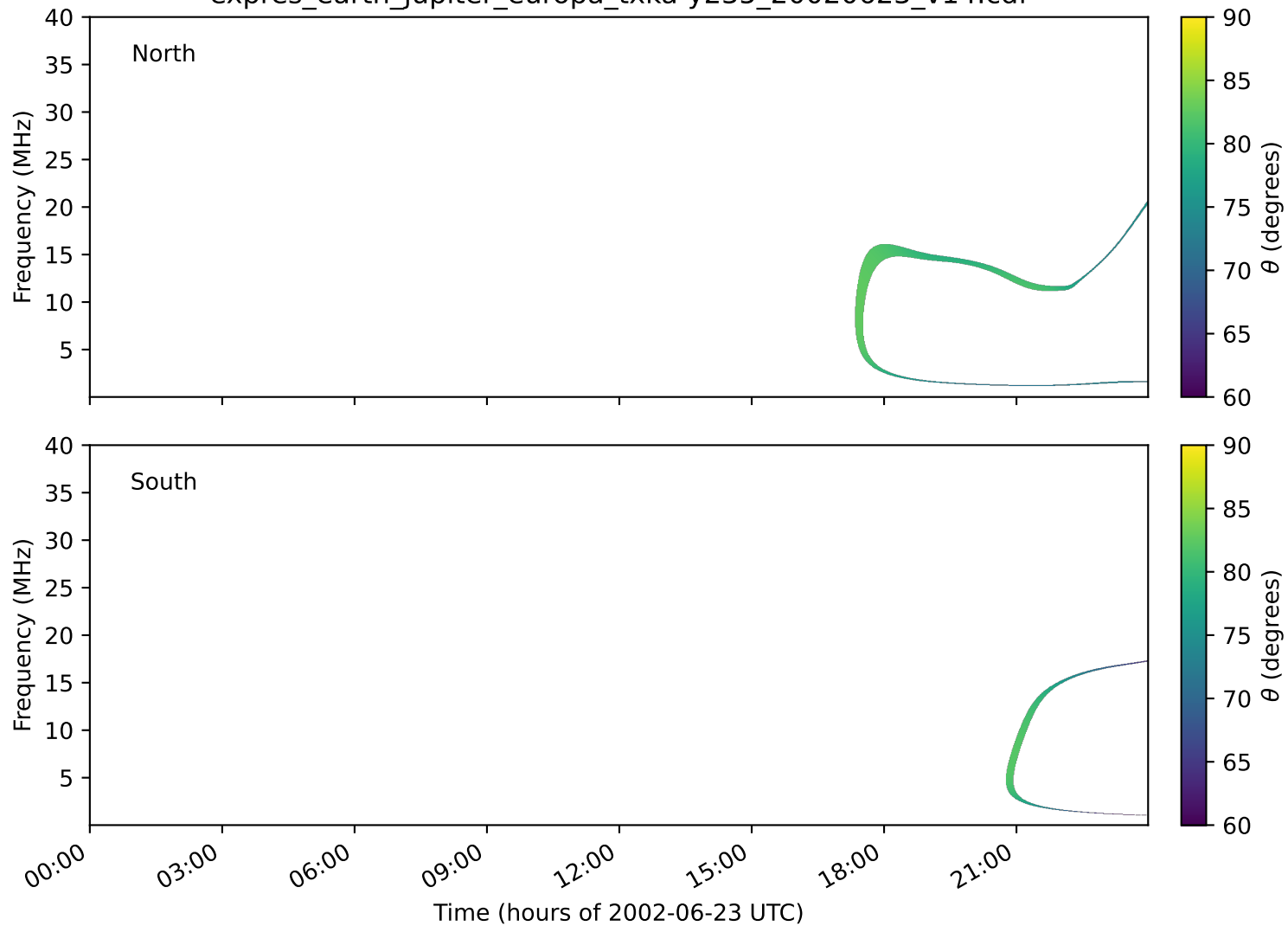
expres_earth_jupiter_europa_txka-y235_20020623_v14.cdf
