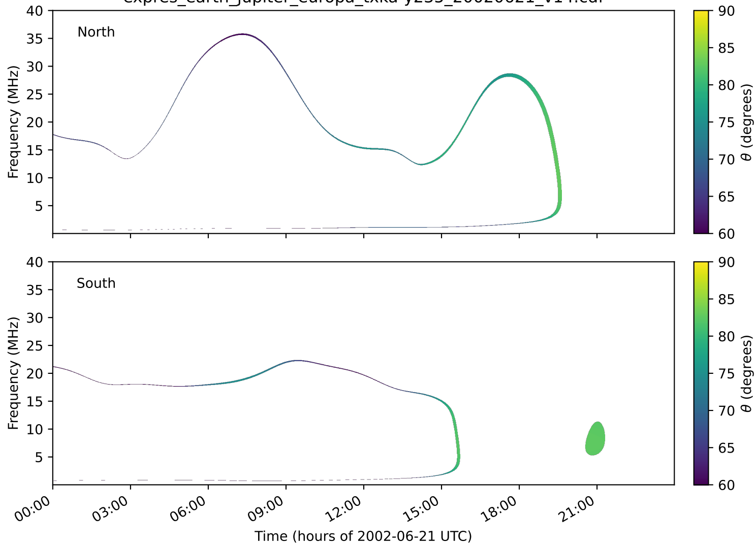
expres_earth_jupiter_europa_txka-y235_20020621_v14.cdf
