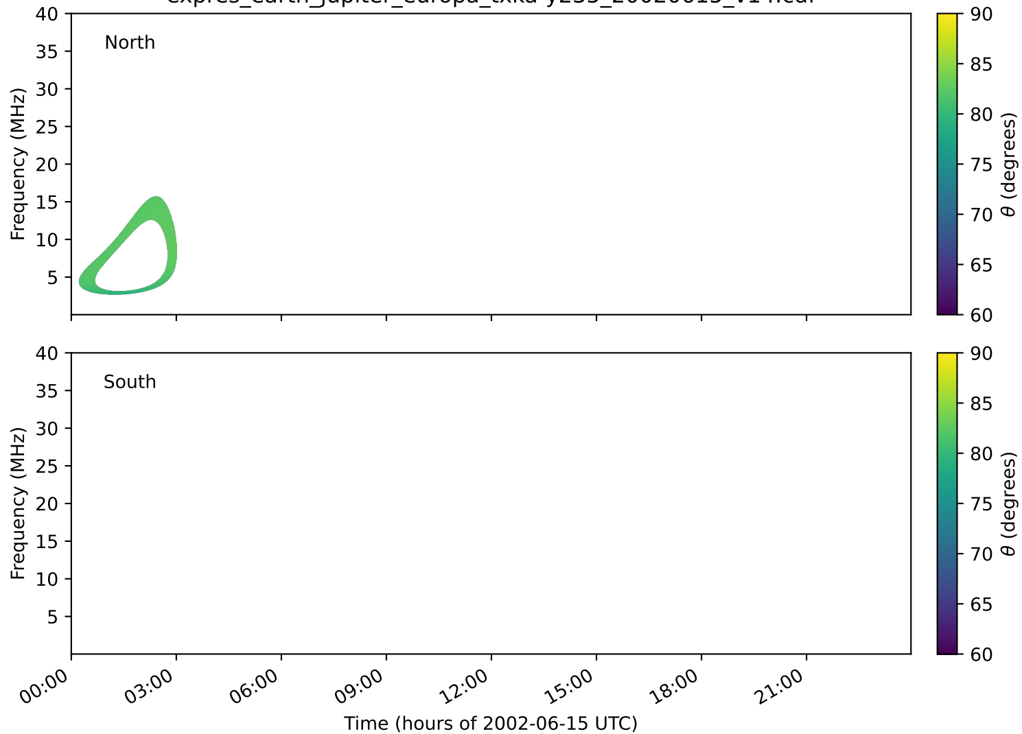
expres_earth_jupiter_europa_txka-y235_20020615_v14.cdf
