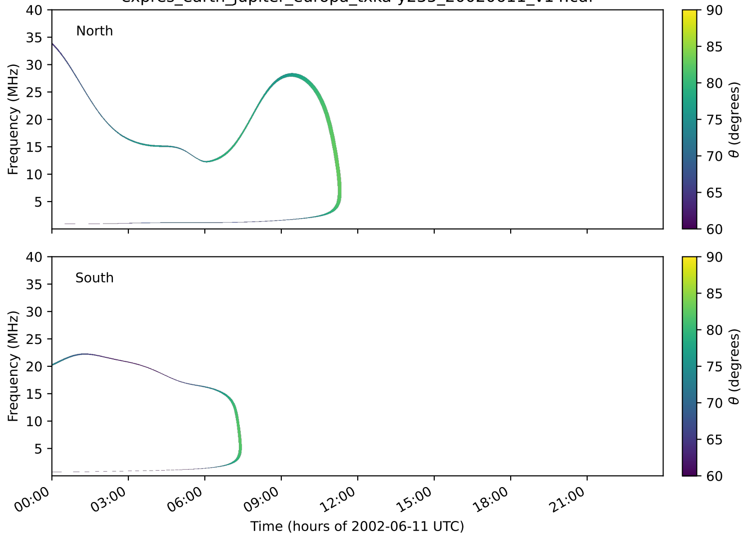
expres_earth_jupiter_europa_txka-y235_20020611_v14.cdf
