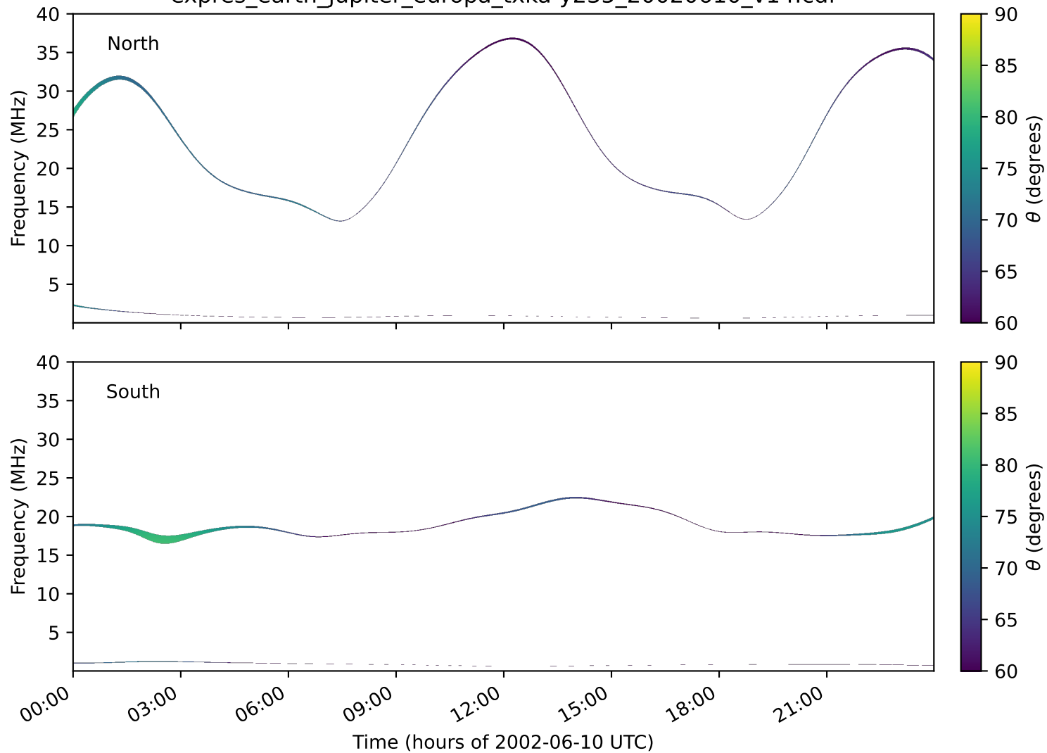
expres_earth_jupiter_europa_txka-y235_20020610_v14.cdf
