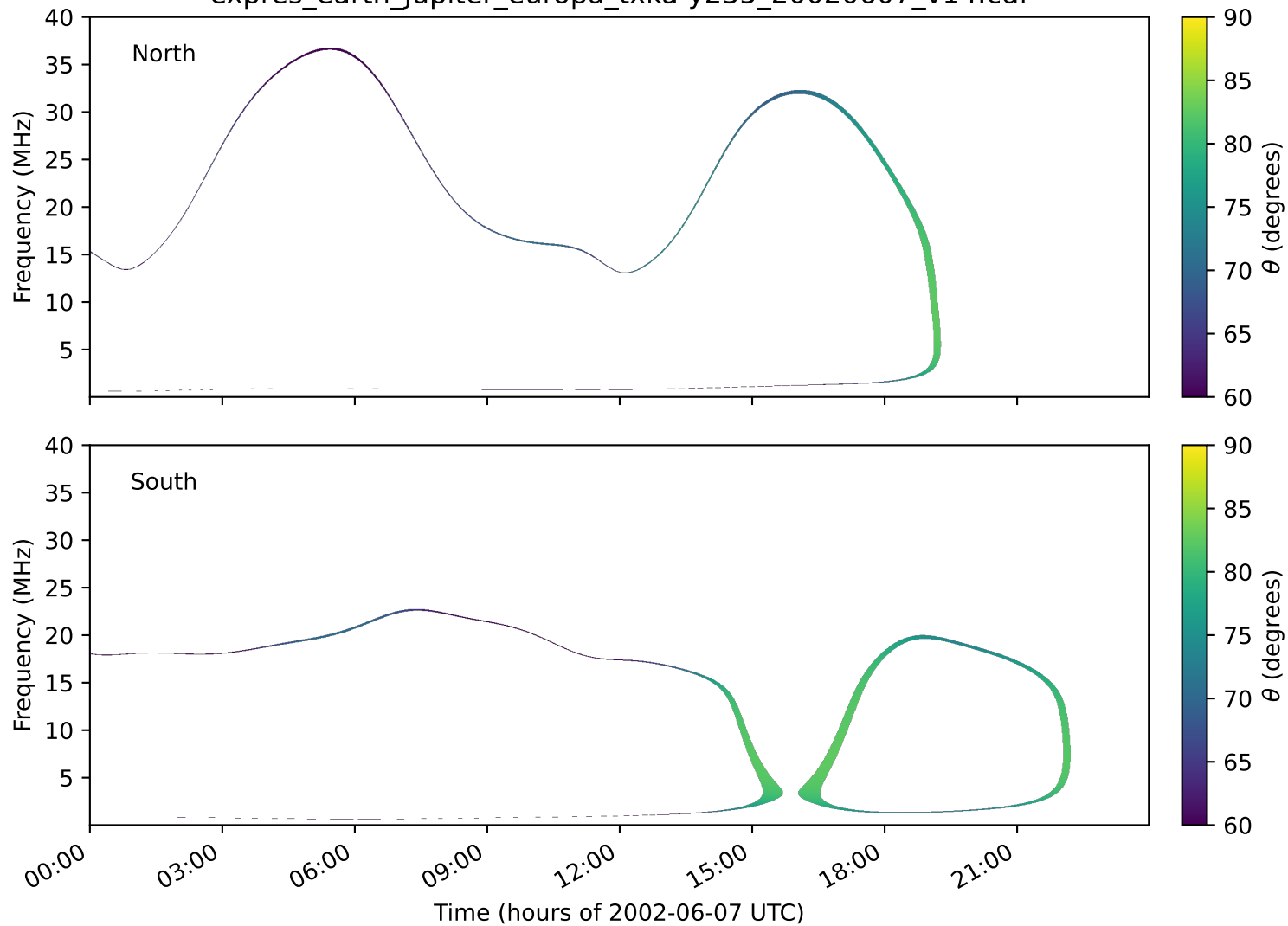
expres_earth_jupiter_europa_txka-y235_20020607_v14.cdf
