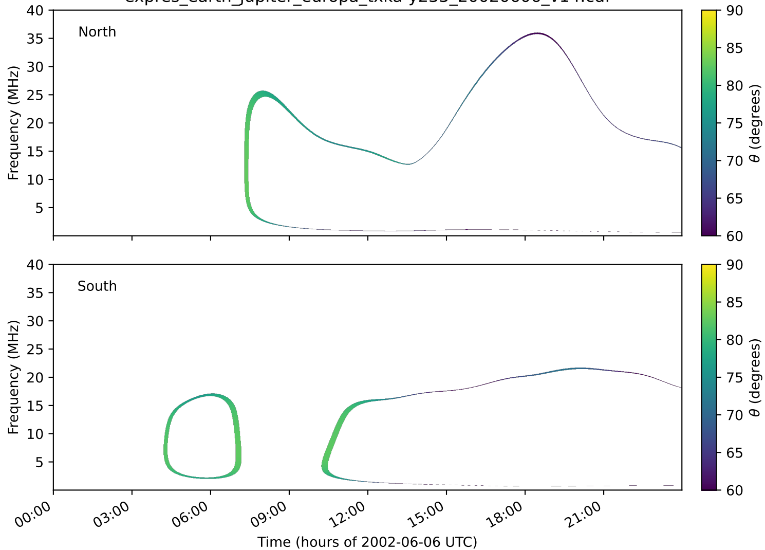
expres_earth_jupiter_europa_txka-y235_20020606_v14.cdf
