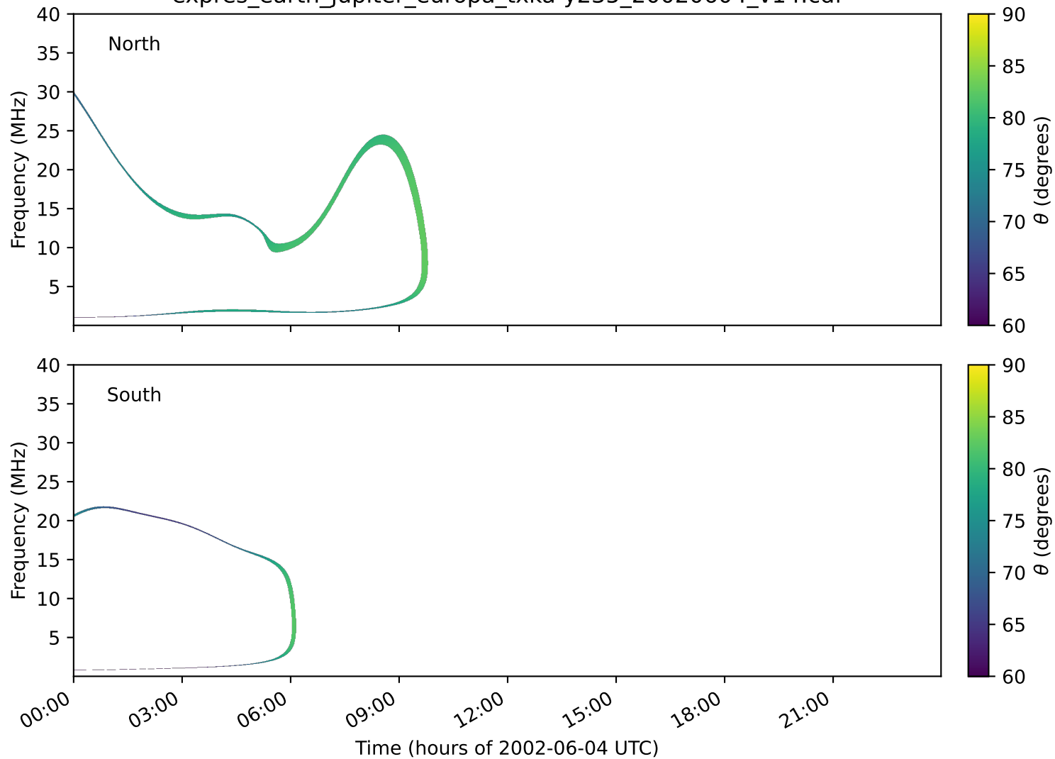
expres_earth_jupiter_europa_txka-y235_20020604_v14.cdf
