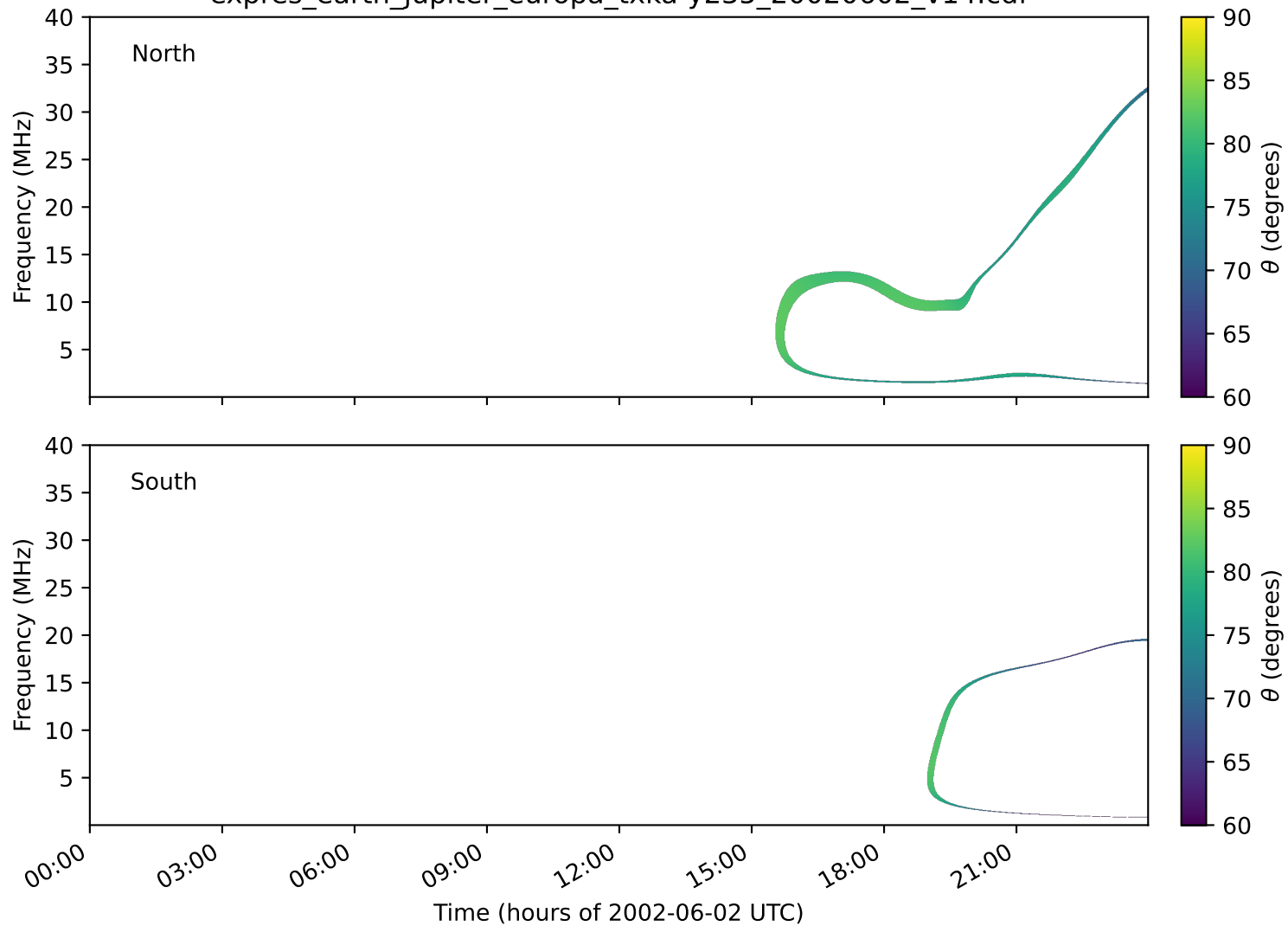
expres_earth_jupiter_europa_txka-y235_20020602_v14.cdf
