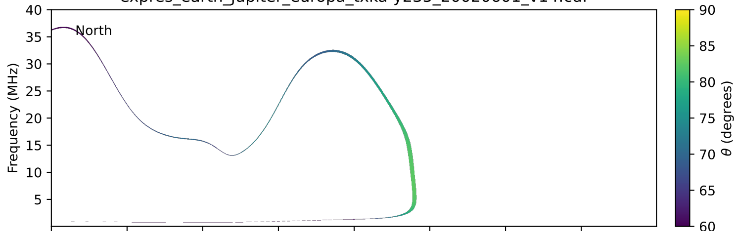
expres_earth_jupiter_europa_txka-y235_20020601_v14.cdf
