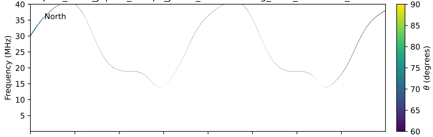
expres_earth_jupiter_europa_jrm33_lossc-wid1deg_3kev_20020617_v11.cdf
