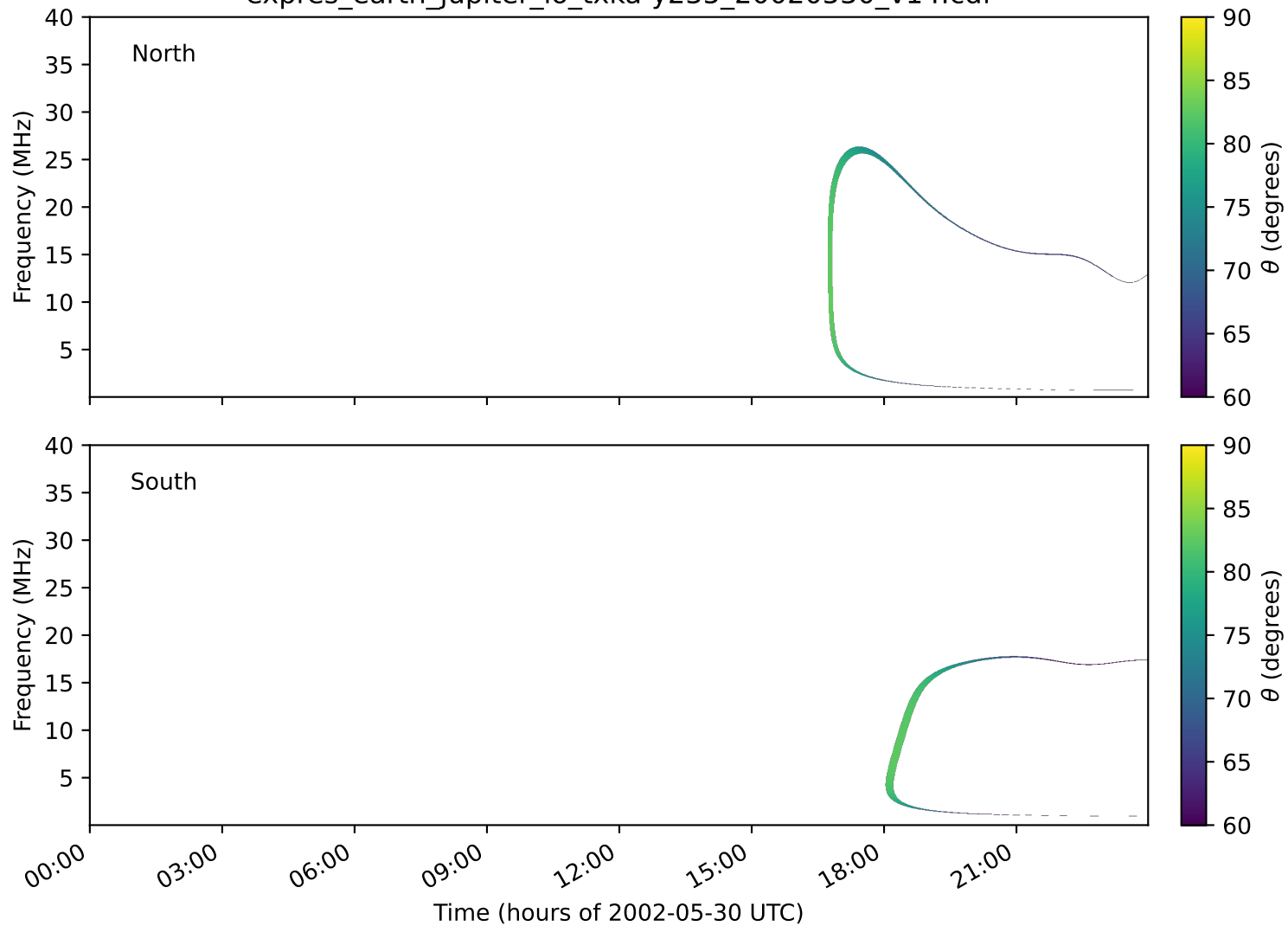
expres_earth_jupiter_io_txka-y235_20020530_v14.cdf
