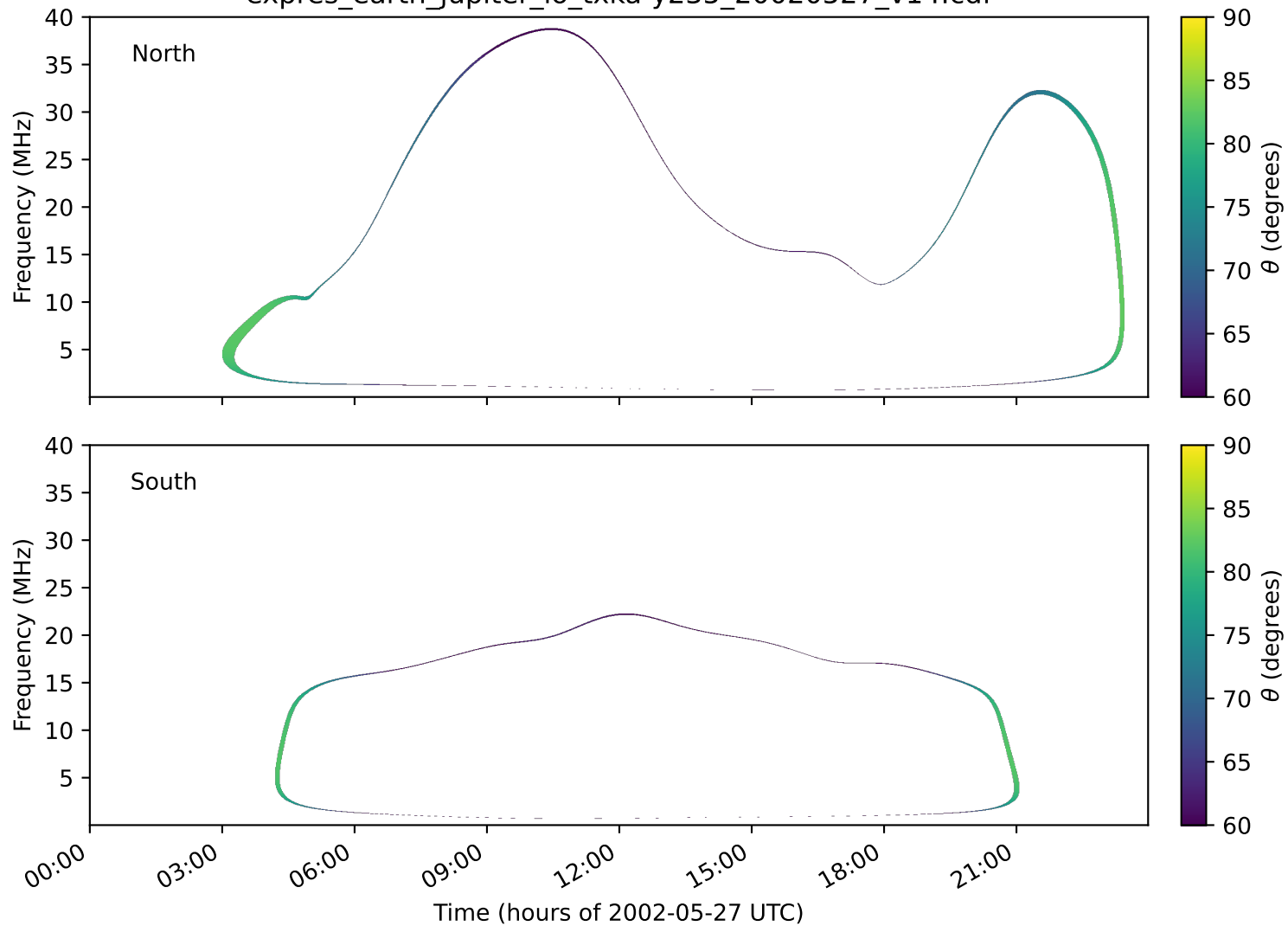
expres_earth_jupiter_io_txka-y235_20020527_v14.cdf
