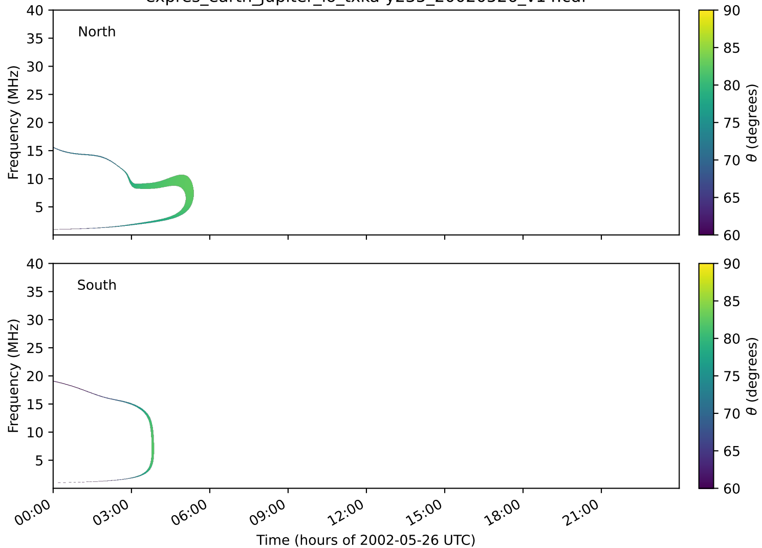
expres_earth_jupiter_io_txka-y235_20020526_v14.cdf
