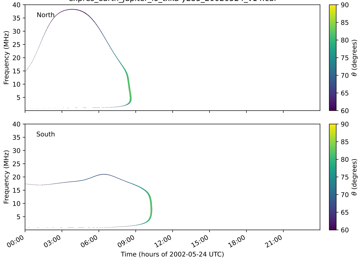
expres_earth_jupiter_io_txka-y235_20020524_v14.cdf
