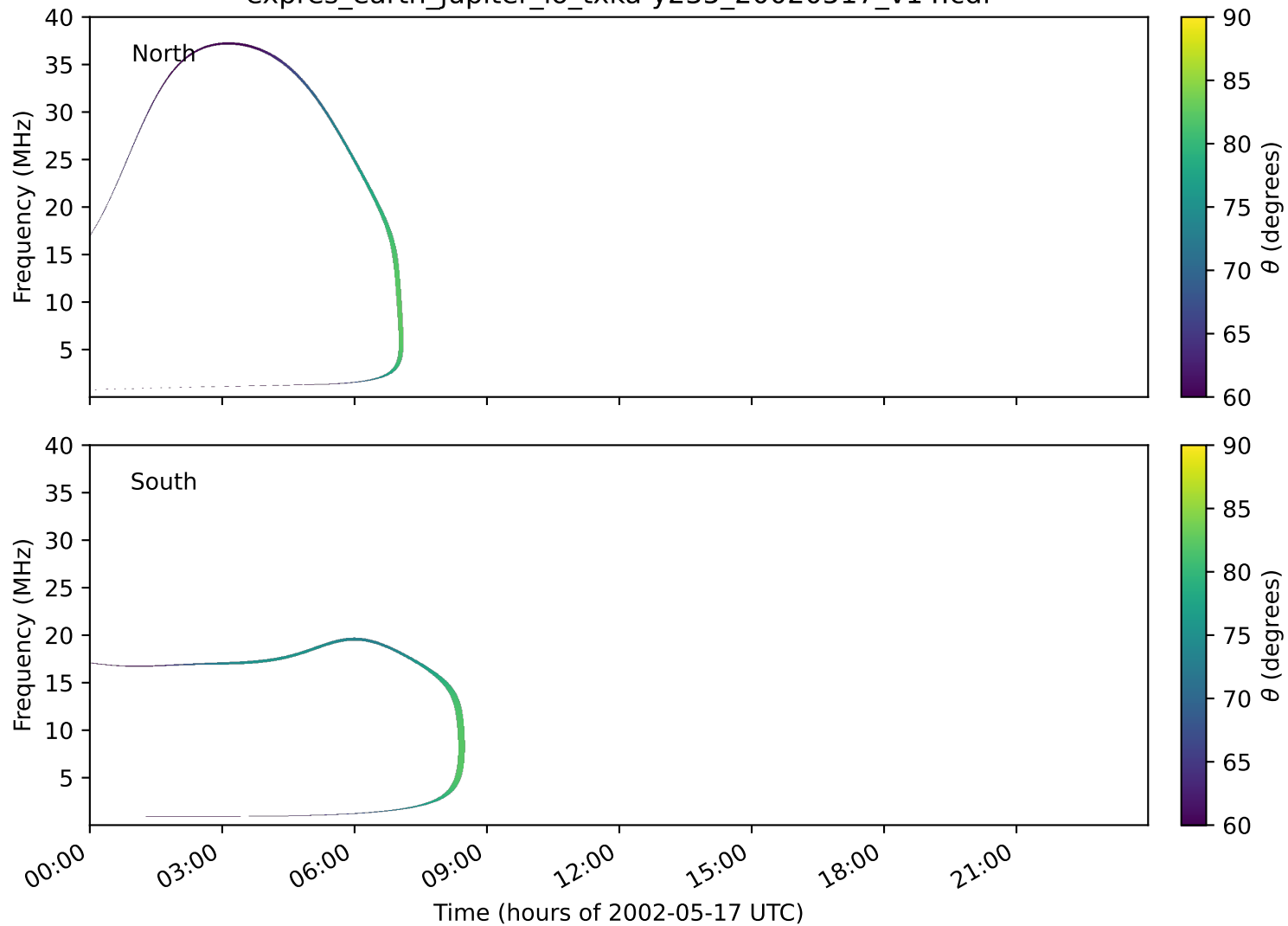
expres_earth_jupiter_io_txka-y235_20020517_v14.cdf
