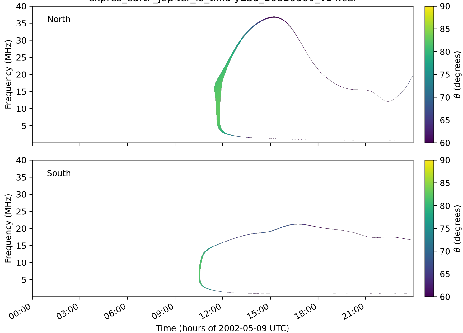
expres_earth_jupiter_io_txka-y235_20020509_v14.cdf
