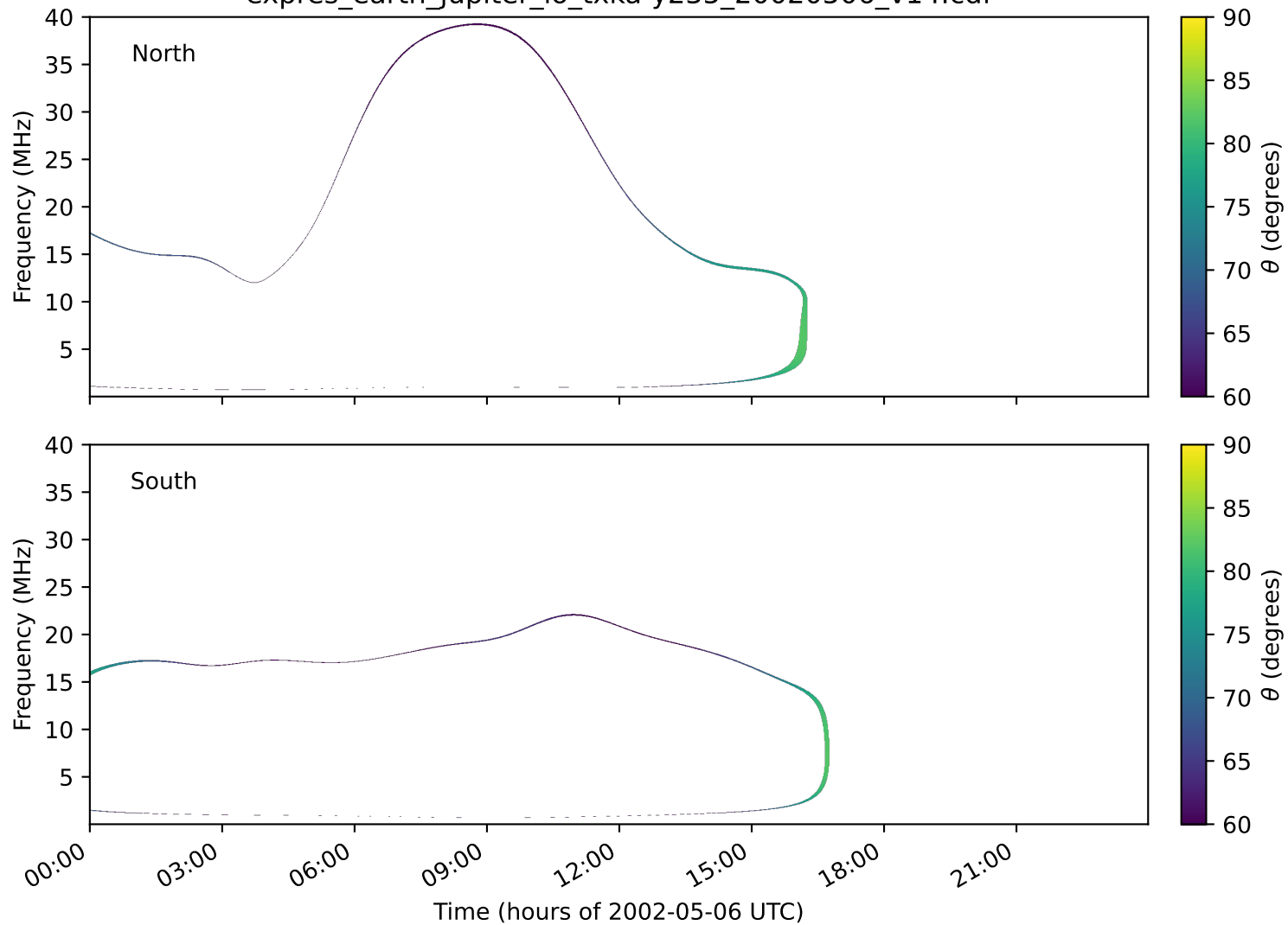
expres_earth_jupiter_io_txka-y235_20020506_v14.cdf
