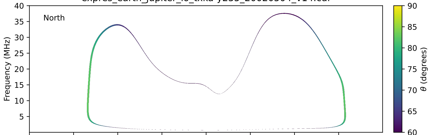
expres_earth_jupiter_io_txka-y235_20020504_v14.cdf
