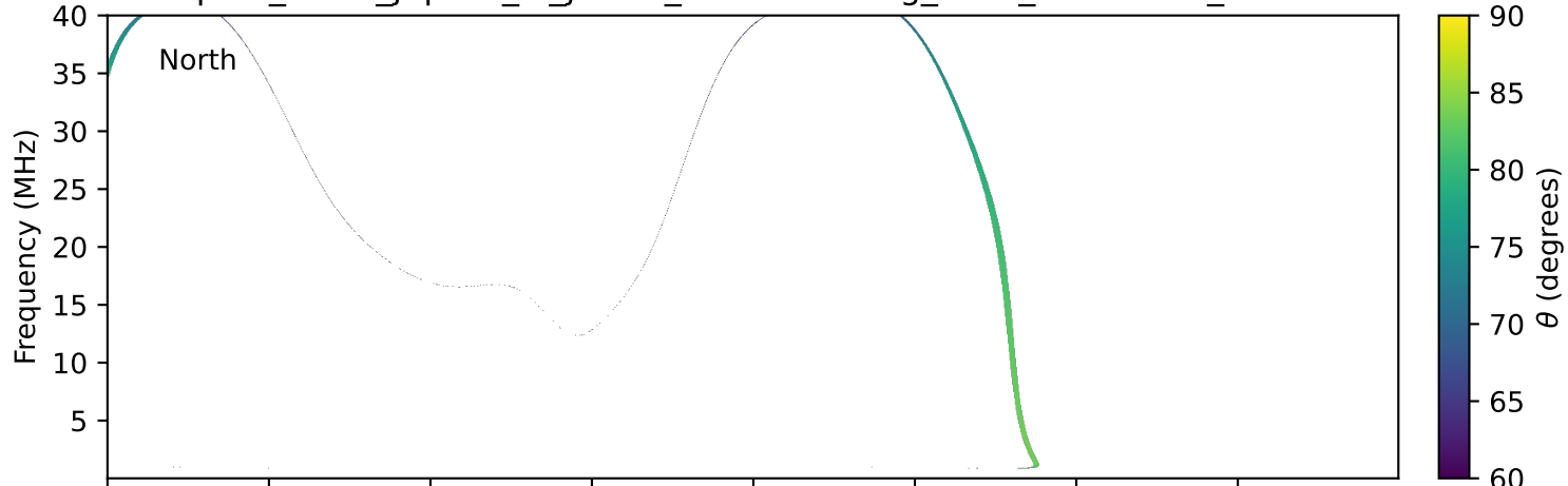
expres_earth_jupiter_io_jrm33_lossc-wid1deg_3kev_20020529_v11.cdf
