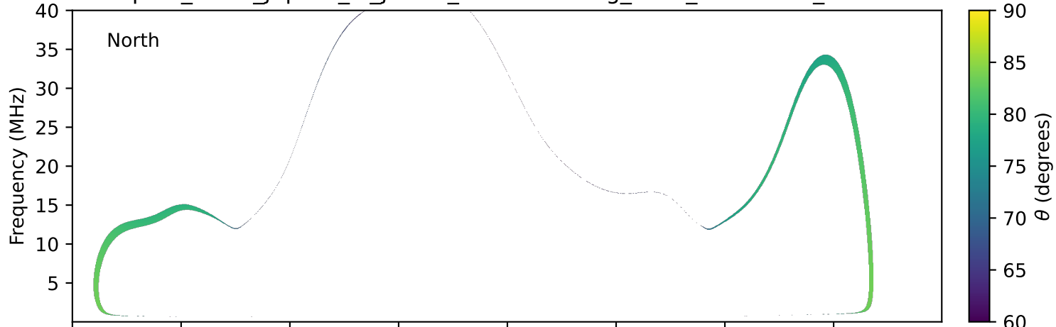
expres_earth_jupiter_io_jrm33_lossc-wid1deg_3kev_20020520_v11.cdf
