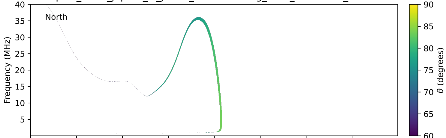
expres_earth_jupiter_io_jrm33_lossc-wid1deg_3kev_20020508_v11.cdf
