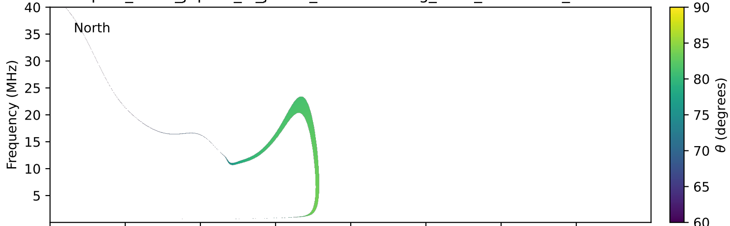
expres_earth_jupiter_io_jrm33_lossc-wid1deg_3kev_20020501_v11.cdf
