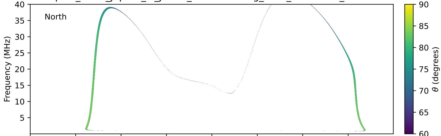
expres_earth_jupiter_io_jrm09_lossc-wid1deg_3kev_20020504_v11.cdf
