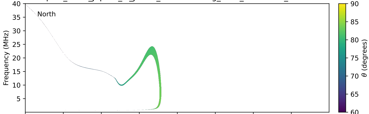
expres_earth_jupiter_io_jrm09_lossc-wid1deg_3kev_20020501_v11.cdf
