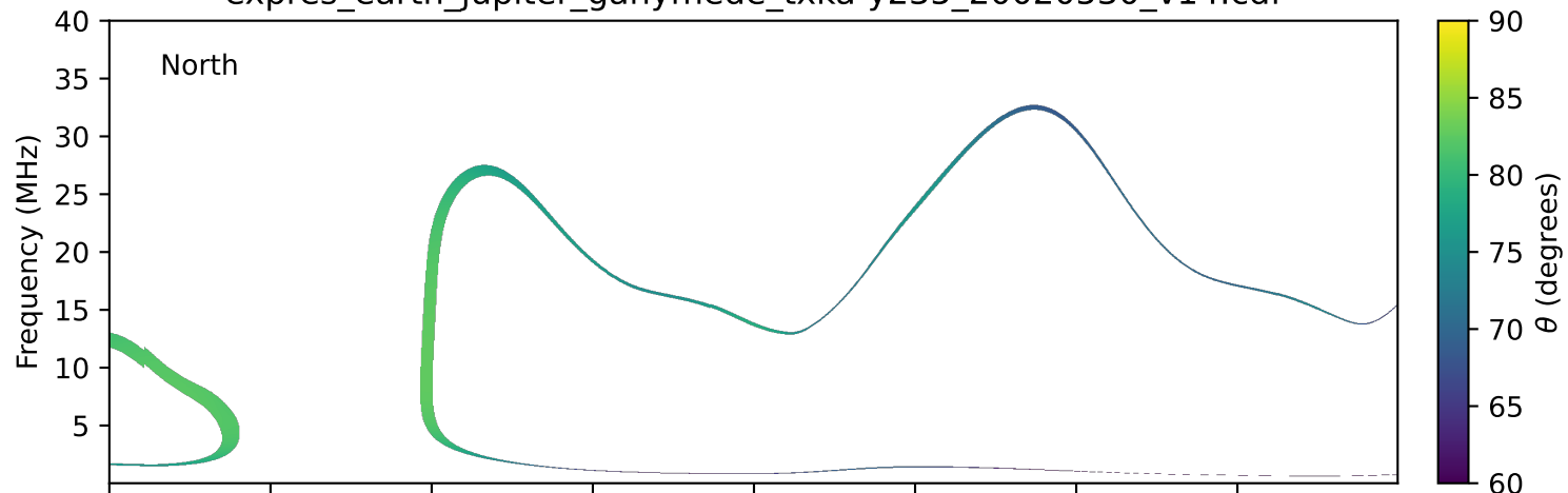
expres_earth_jupiter_ganymede_txka-y235_20020530_v14.cdf
