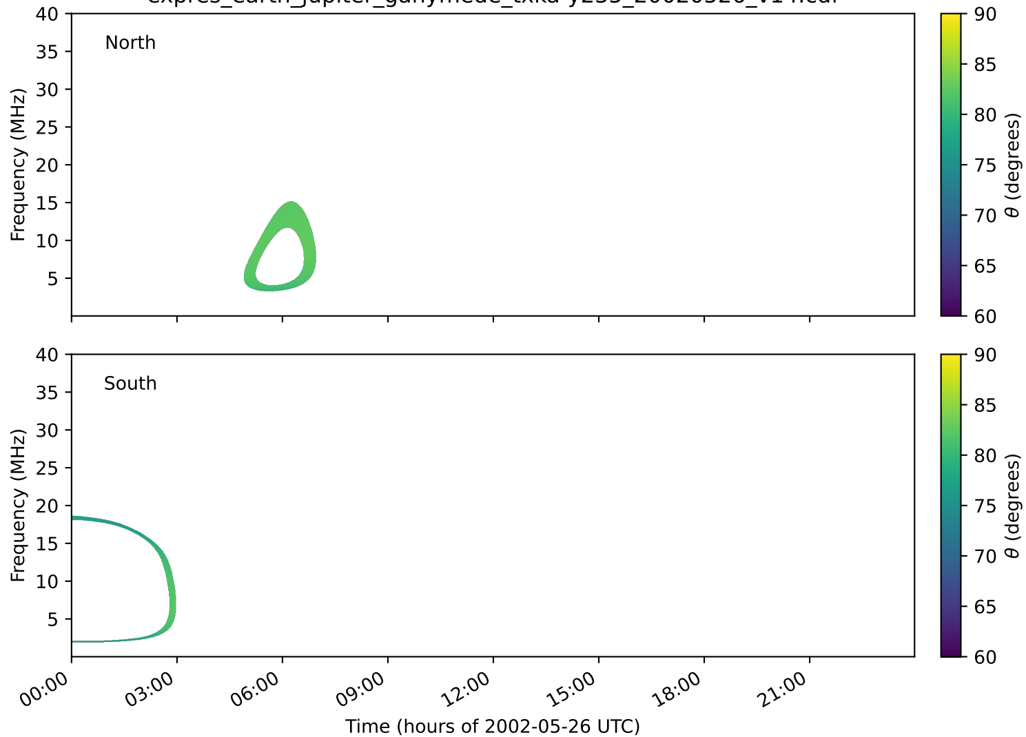
expres_earth_jupiter_ganymede_txka-y235_20020526_v14.cdf
