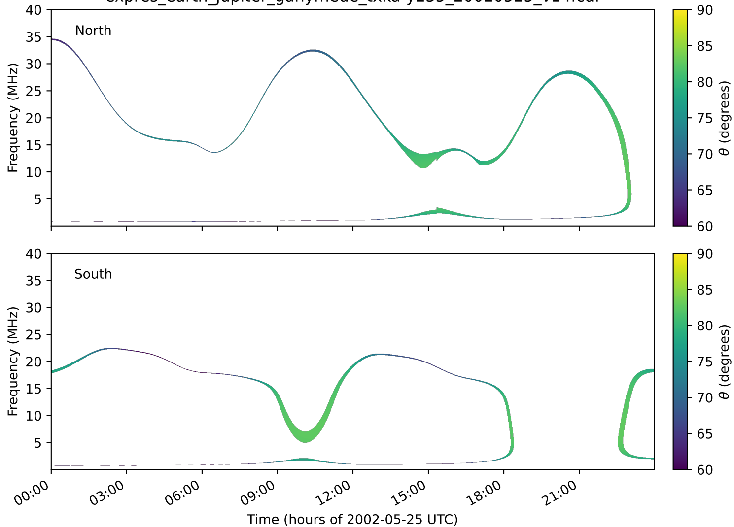
expres_earth_jupiter_ganymede_txka-y235_20020525_v14.cdf
