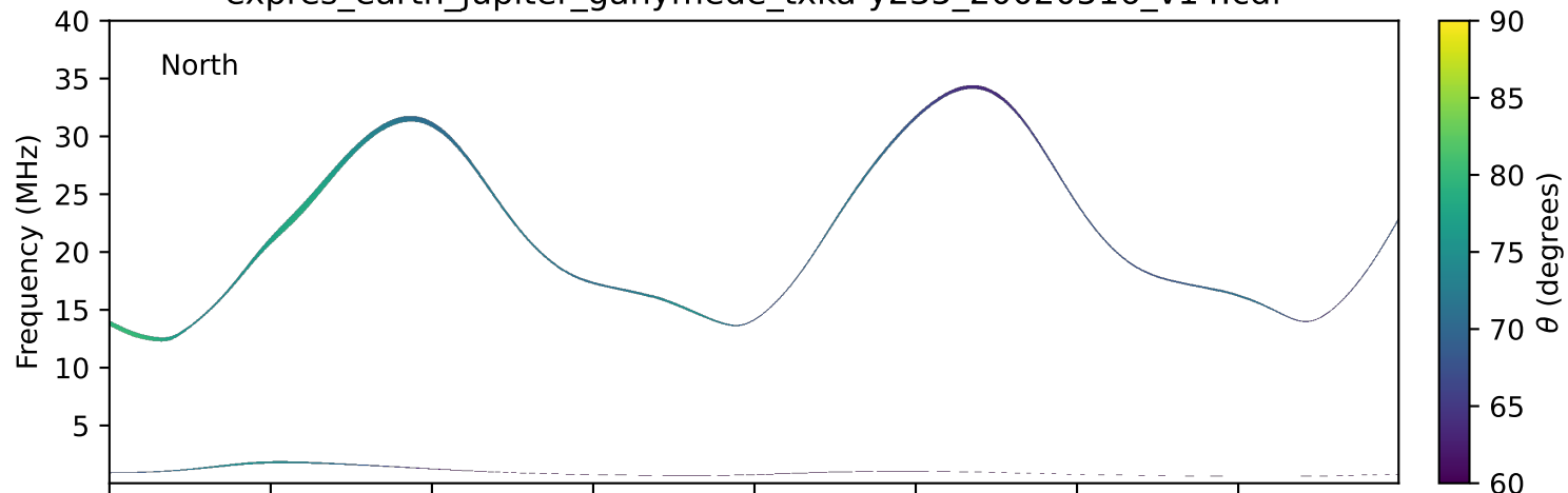
expres_earth_jupiter_ganymede_txka-y235_20020516_v14.cdf
