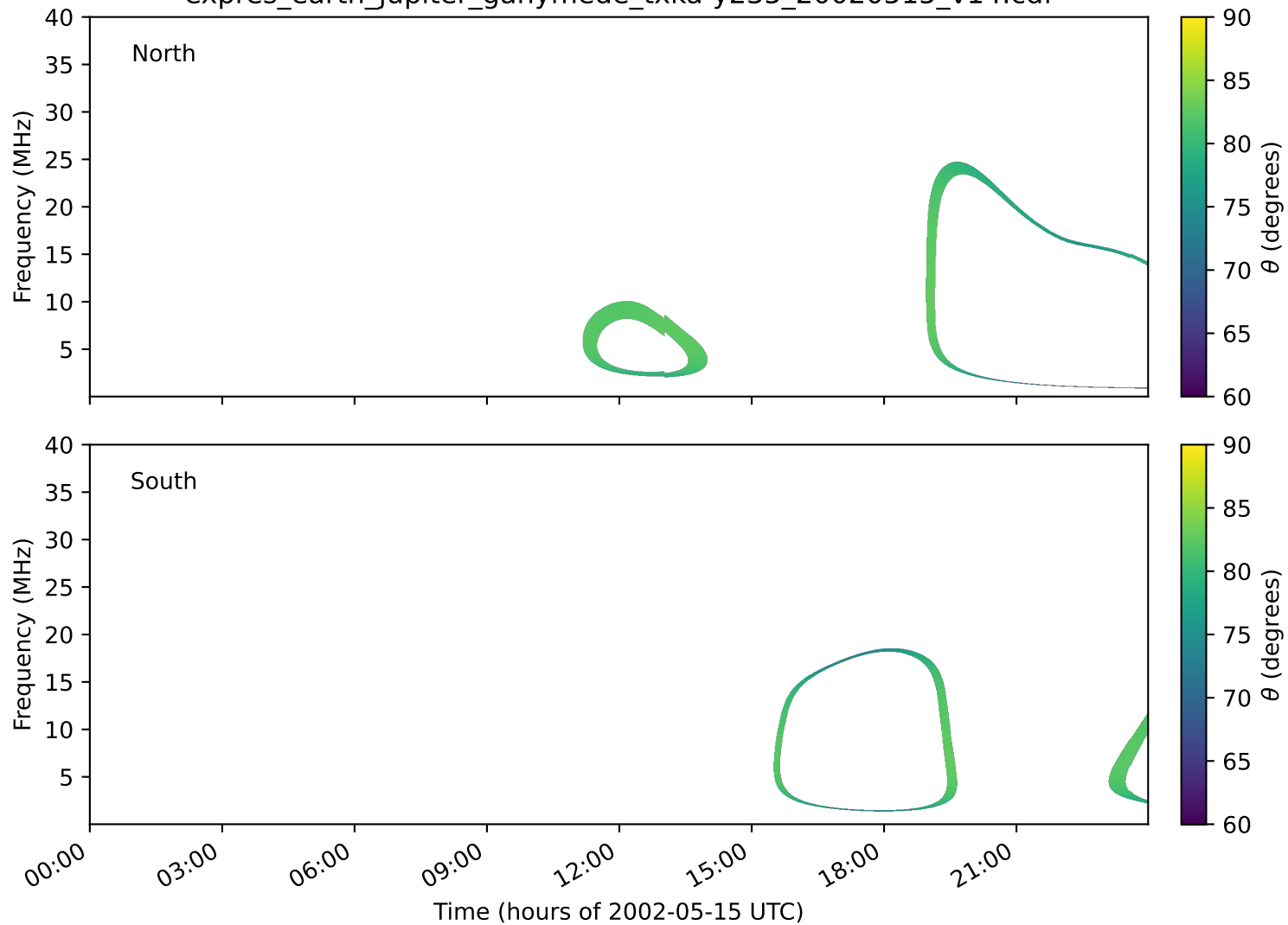
expres_earth_jupiter_ganymede_txka-y235_20020515_v14.cdf
