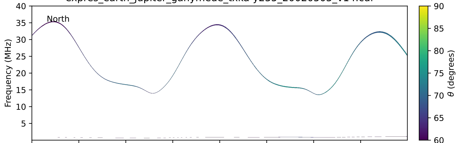
expres_earth_jupiter_ganymede_txka-y235_20020503_v14.cdf
