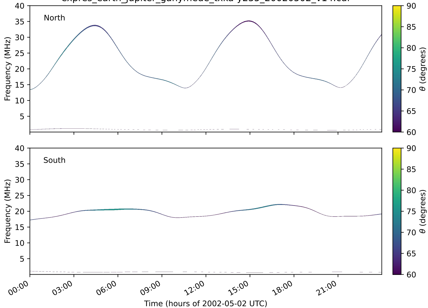
expres_earth_jupiter_ganymede_txka-y235_20020502_v14.cdf
