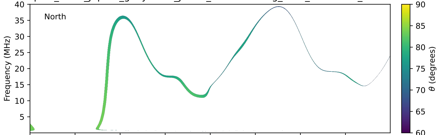
expres_earth_jupiter_ganymede_jrm33_lossc-wid1deg_3kev_20020523_v11.cdf
