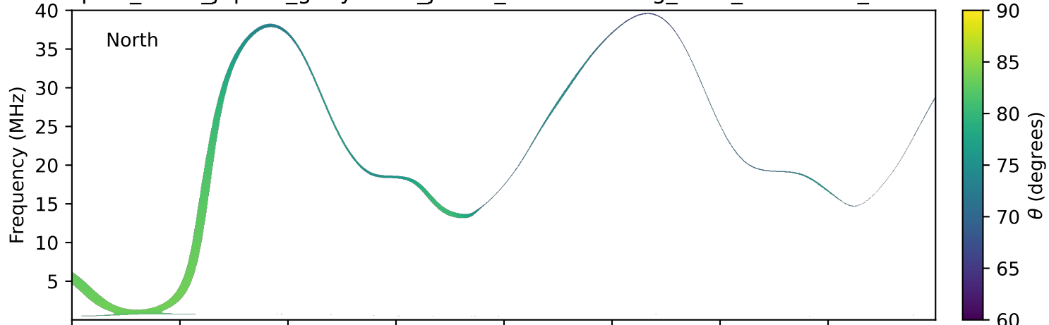
expres_earth_jupiter_ganymede_jrm33_lossc-wid1deg_3kev_20020516_v11.cdf
