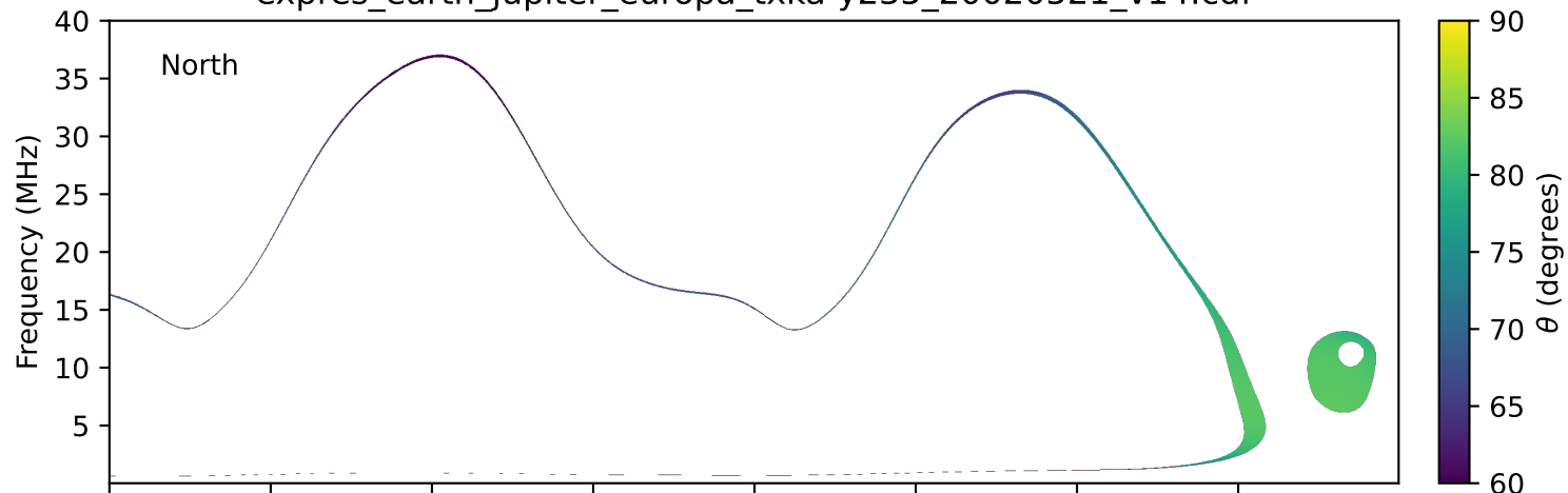
expres_earth_jupiter_europa_txka-y235_20020521_v14.cdf
