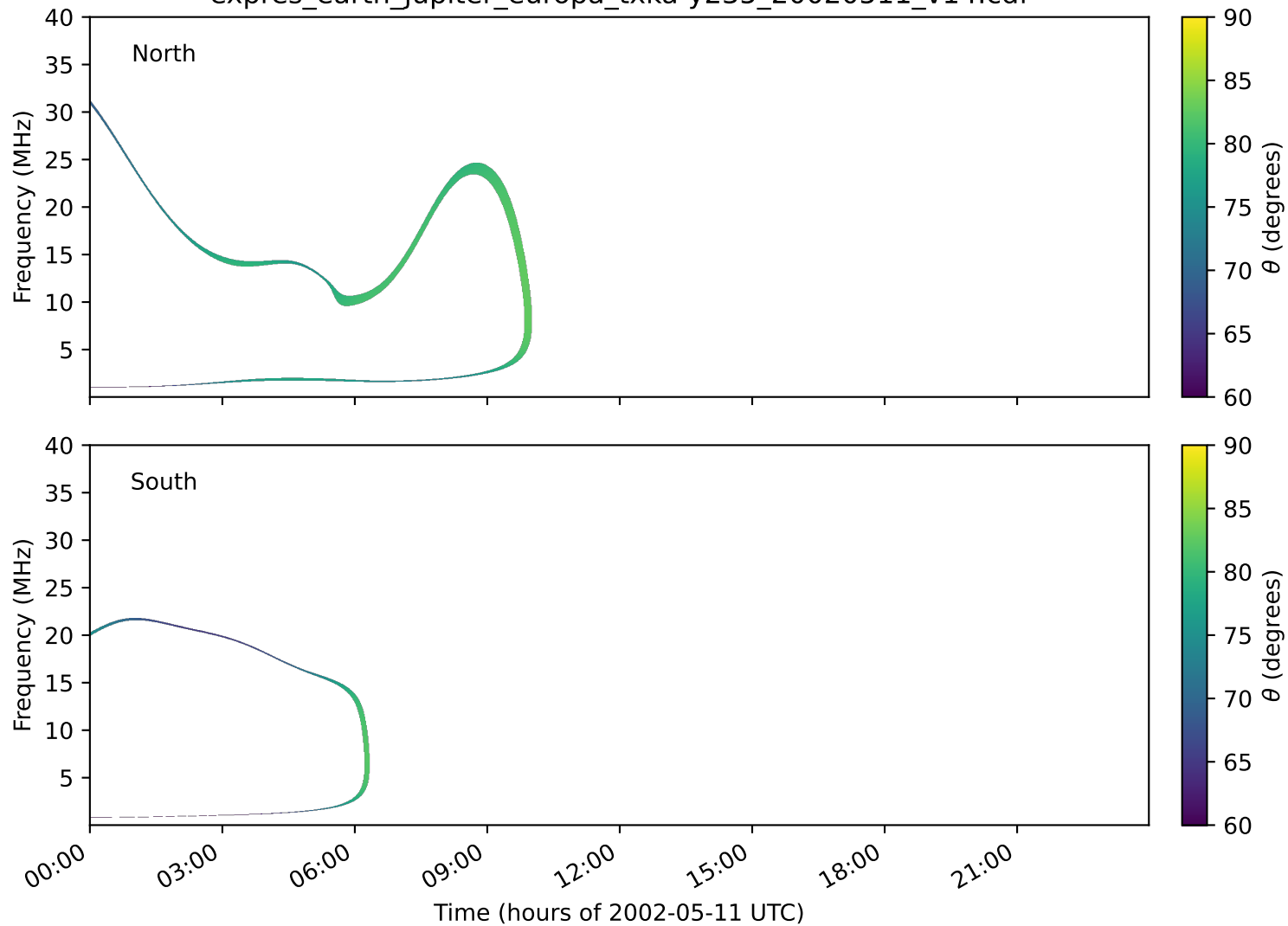
expres_earth_jupiter_europa_txka-y235_20020511_v14.cdf
