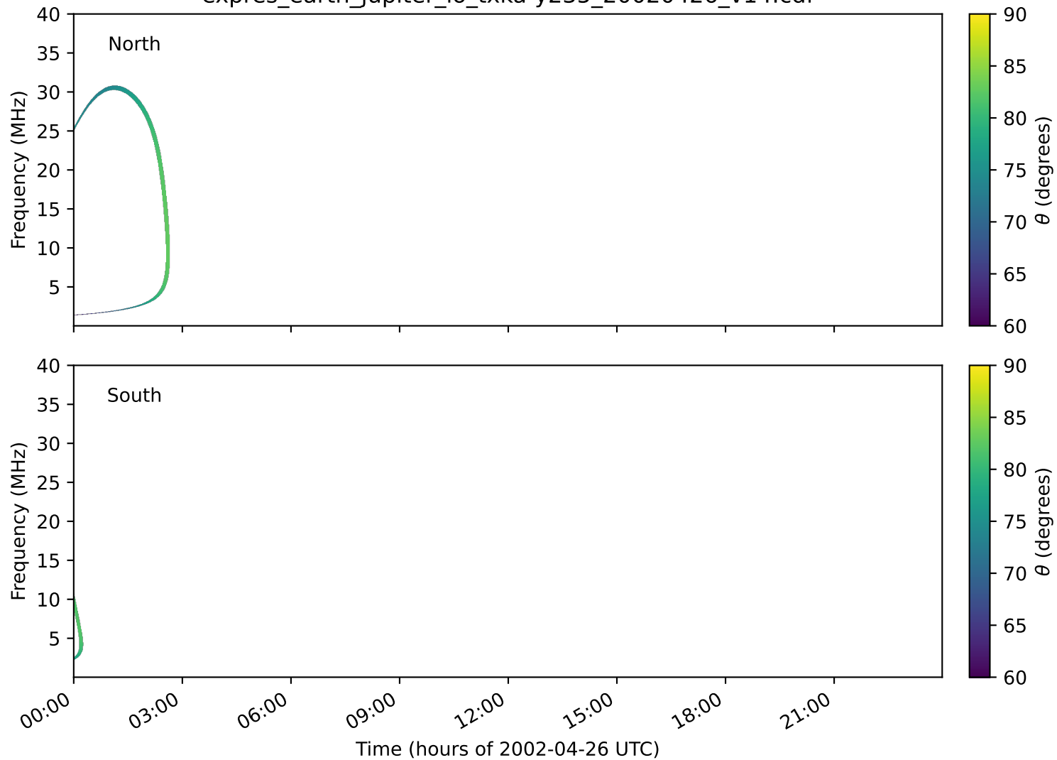
expres_earth_jupiter_io_txka-y235_20020426_v14.cdf
