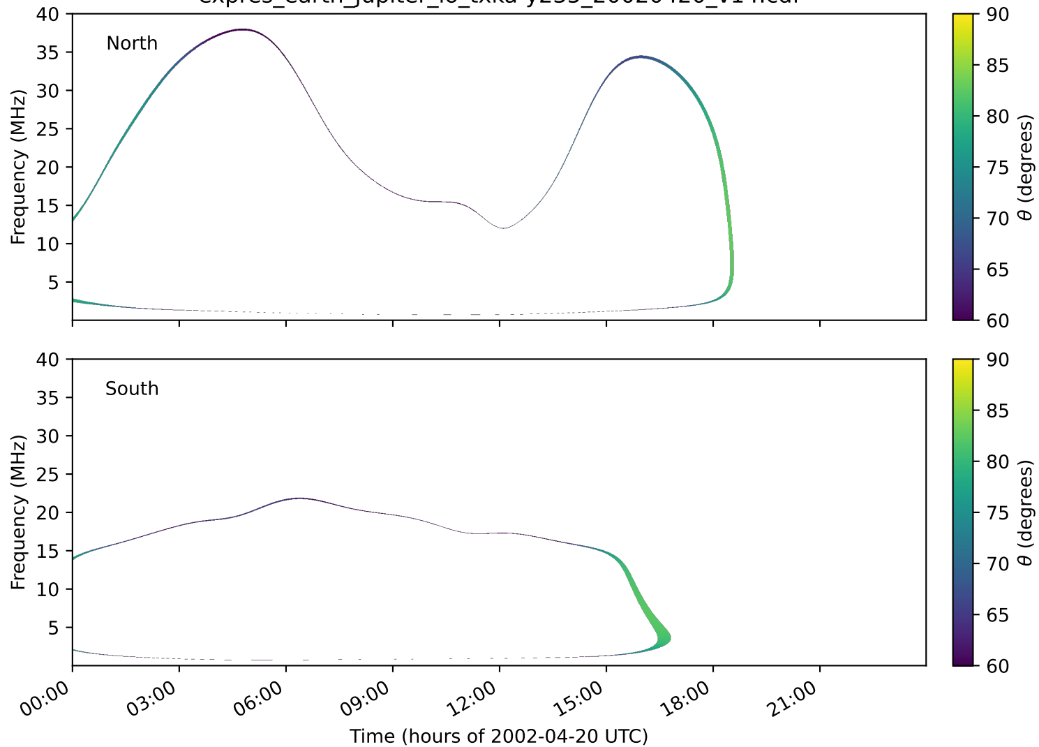
expres_earth_jupiter_io_txka-y235_20020420_v14.cdf
