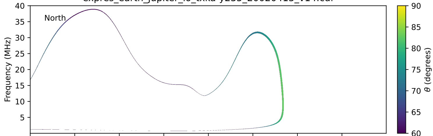
expres_earth_jupiter_io_txka-y235_20020413_v14.cdf
