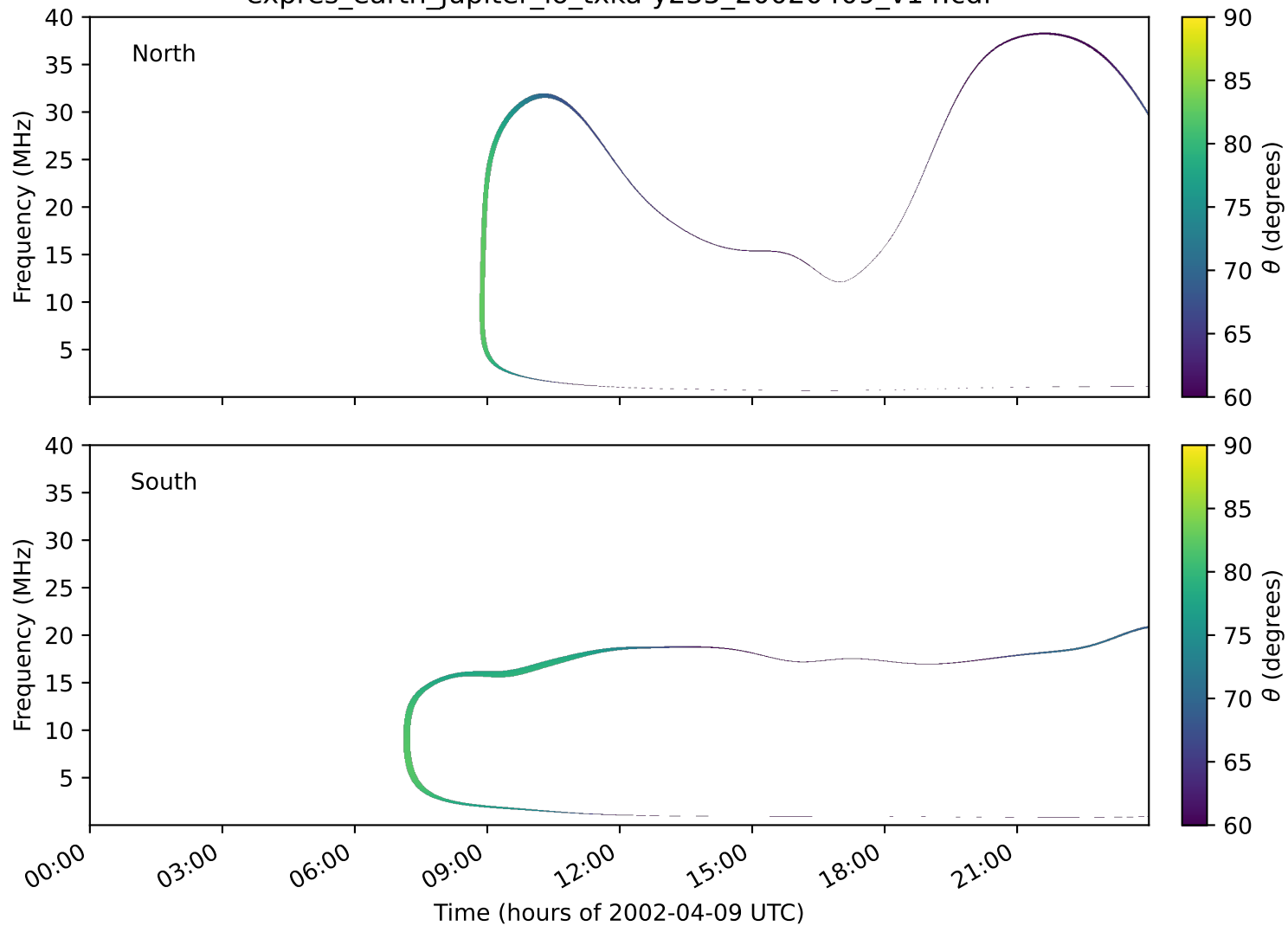
expres_earth_jupiter_io_txka-y235_20020409_v14.cdf
