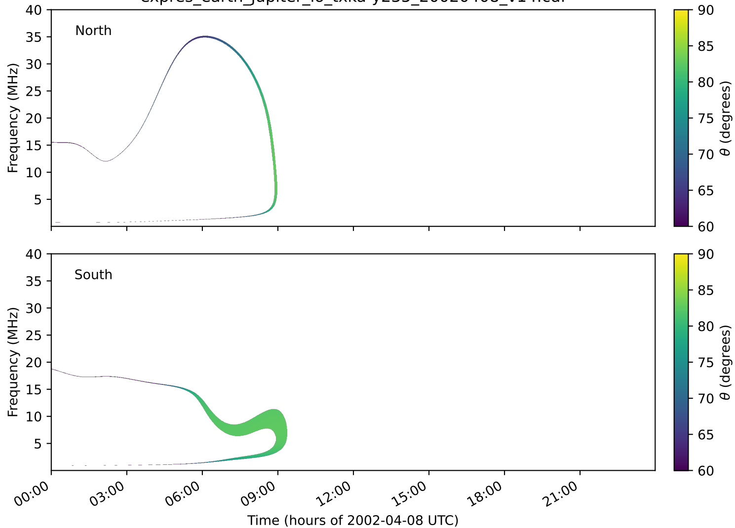
expres_earth_jupiter_io_txka-y235_20020408_v14.cdf
