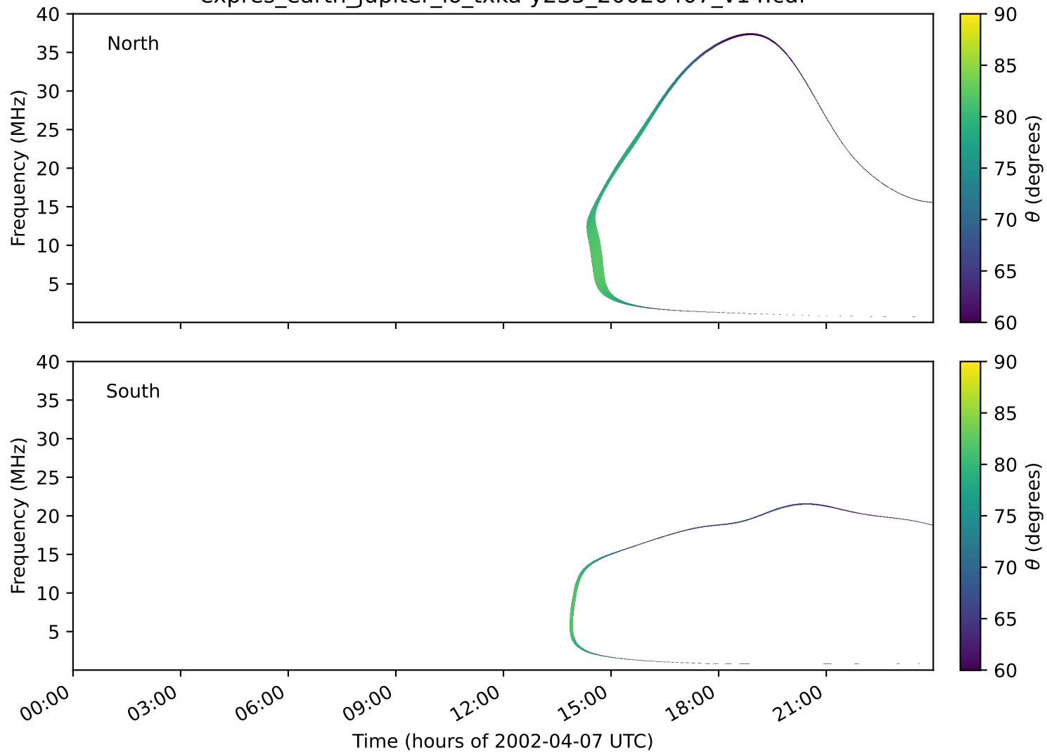
expres_earth_jupiter_io_txka-y235_20020407_v14.cdf
