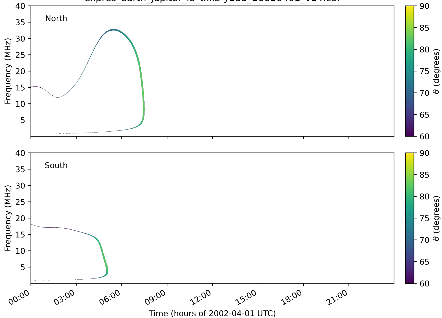
expres_earth_jupiter_io_txka-y235_20020401_v14.cdf
