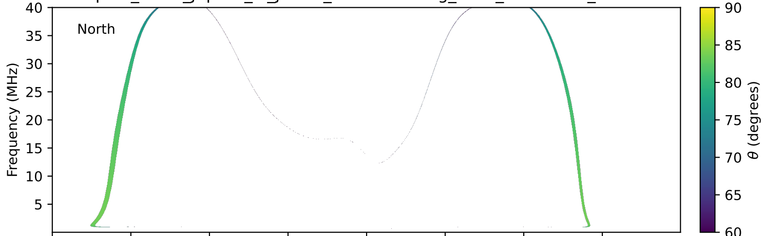
expres_earth_jupiter_io_jrm33_lossc-wid1deg_3kev_20020427_v11.cdf
