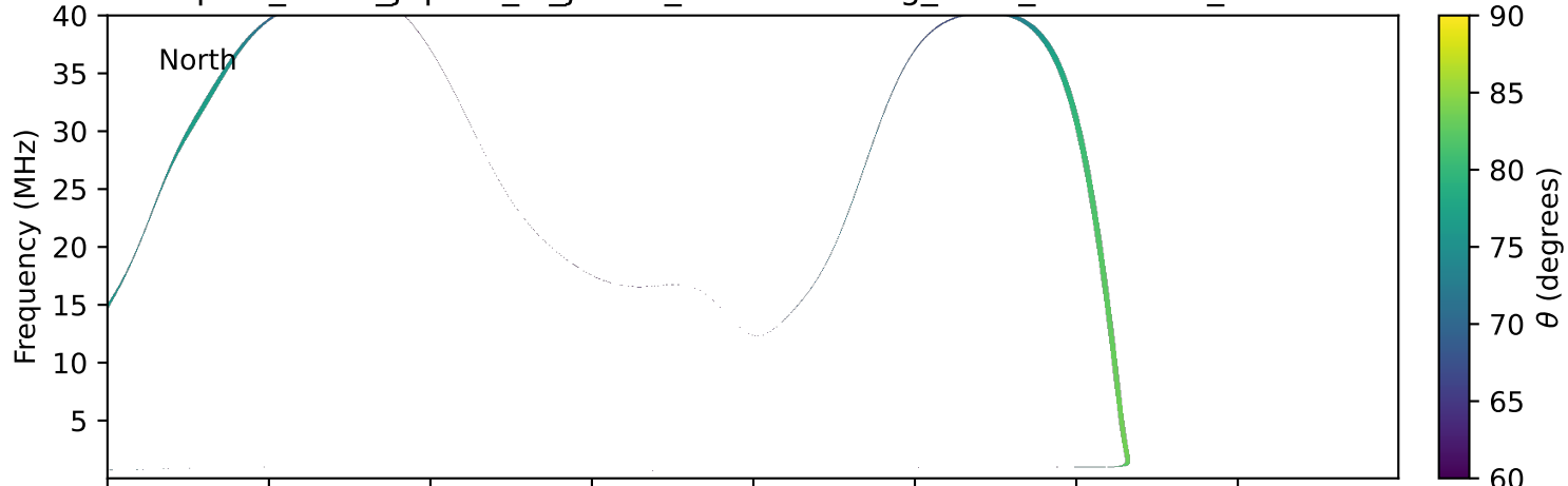
expres_earth_jupiter_io_jrm33_lossc-wid1deg_3kev_20020420_v11.cdf
