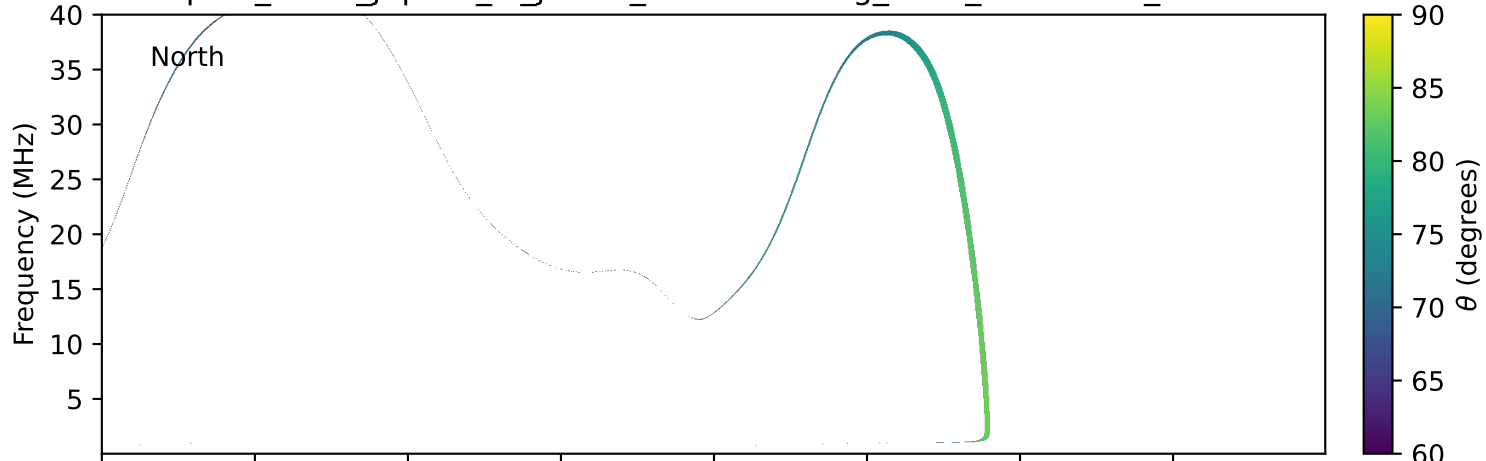
expres_earth_jupiter_io_jrm33_lossc-wid1deg_3kev_20020413_v11.cdf
