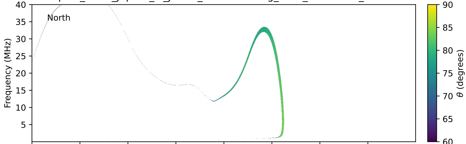
expres_earth_jupiter_io_jrm33_lossc-wid1deg_3kev_20020406_v11.cdf
